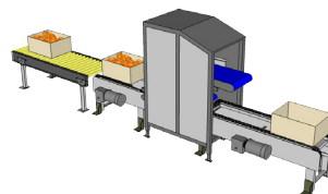
3d scheme for a carton filler simple configuration
