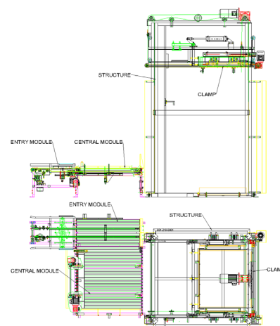
Tray multiformat palletizer parts
